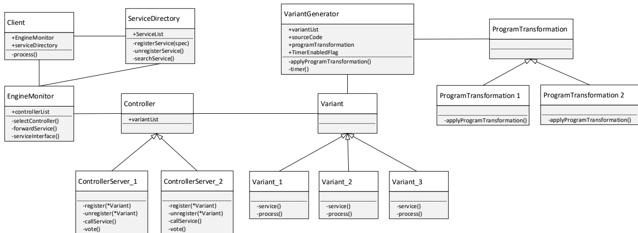
Figure 2. Class diagram of the K-variant architecture for web services.
