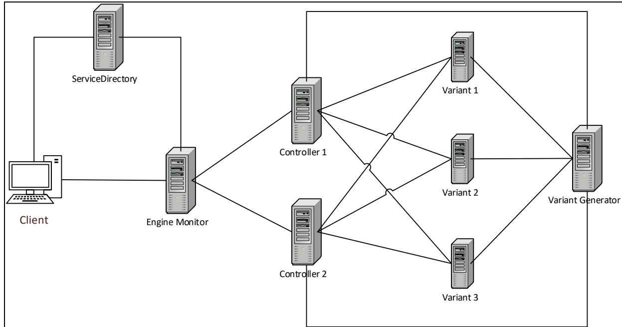
Figure 1 K-variant architecture for web services and applications.
