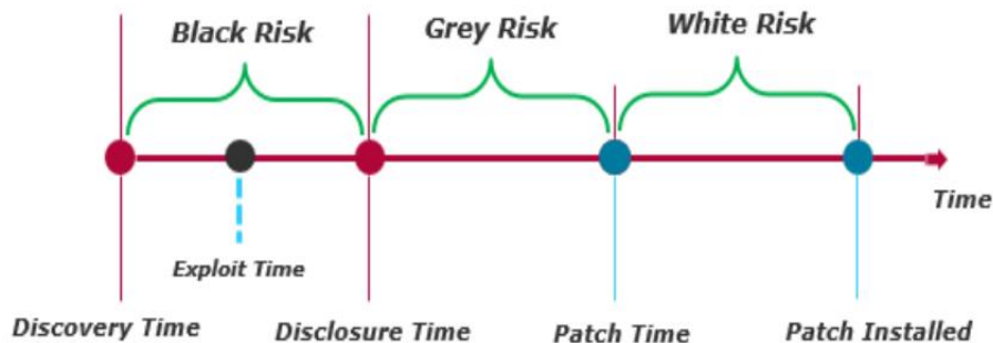
Figure 1: Vulnerability Lifecycle.
