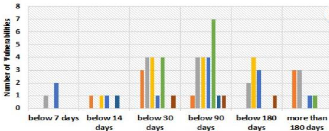
Figure 2: vulnerabilities that are patched after Disclosure Time for OpenStack releases
